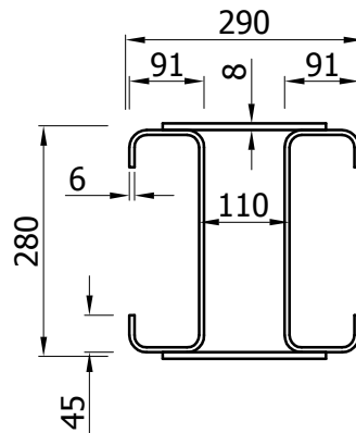
Typical Section
